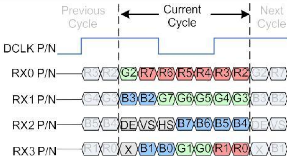
4 Lane JEIDA Data Format Color Bit Map
