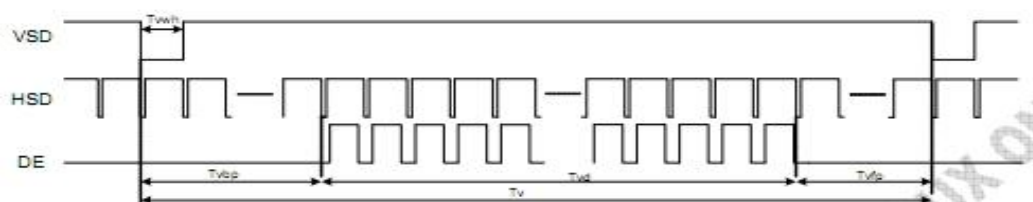
Vertical input timing
