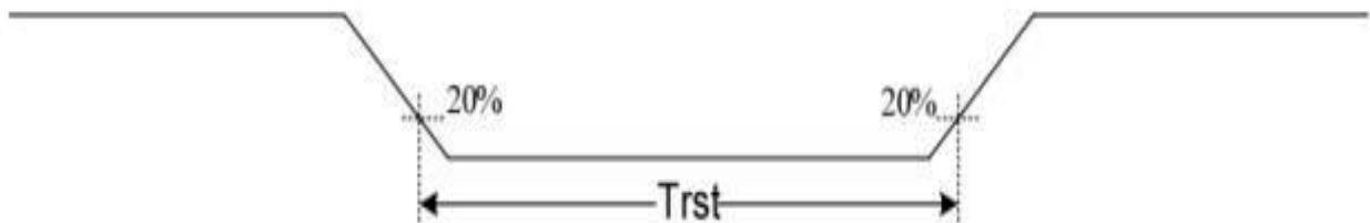
Figure 13.5: Reset timing
