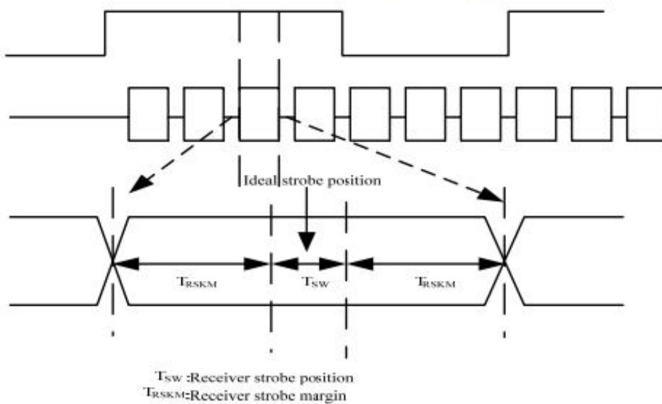
LVDS timing(2)
