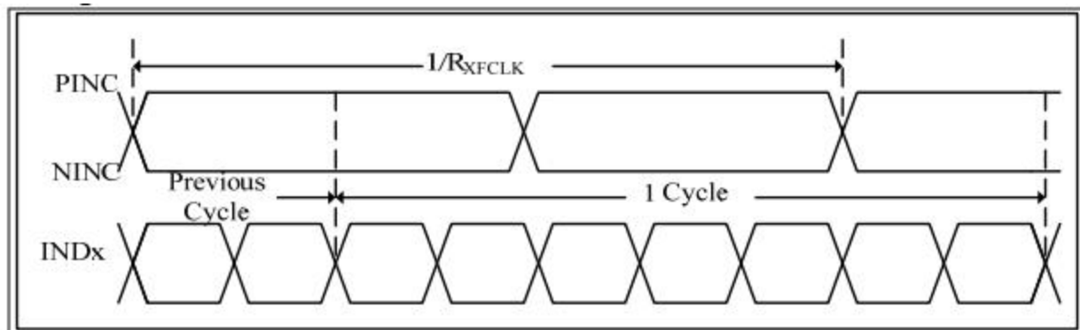
LVDS timing(1)
