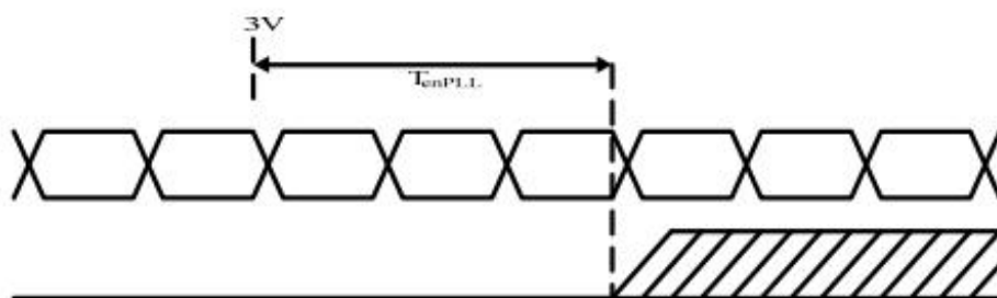
LVDS timing(2)
