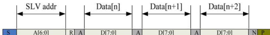
Figure 2-6 I2C master read, slave write
