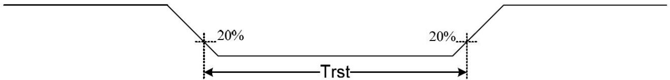
Figure 5.2.1: Reset timing
