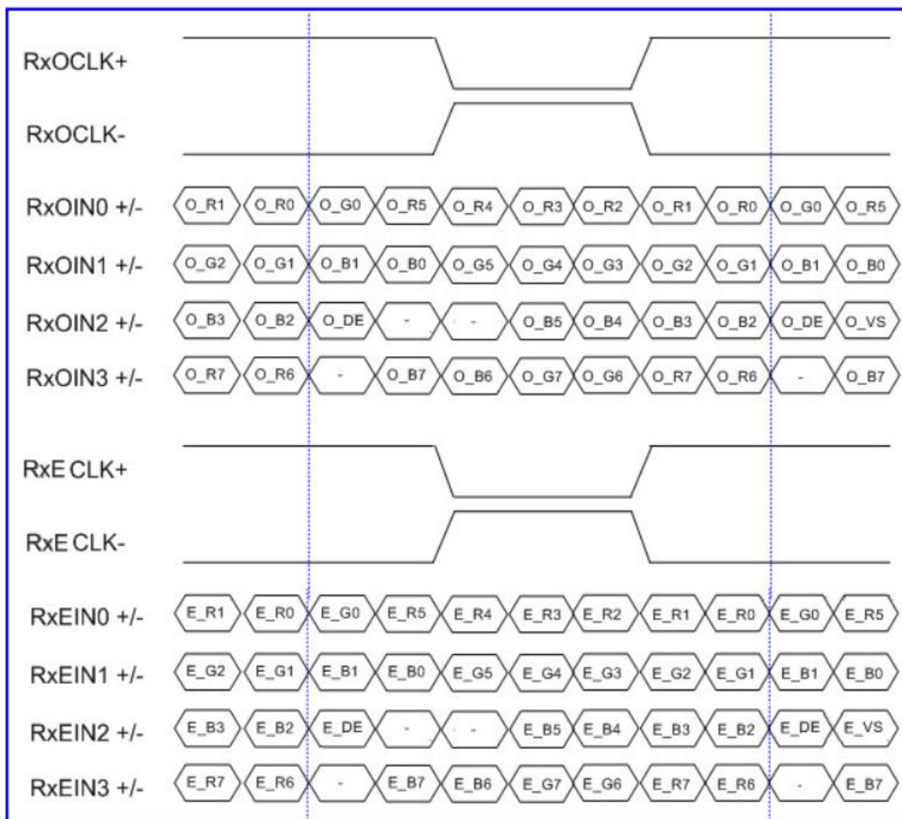
Fig.1 LVDS input data VESA format
