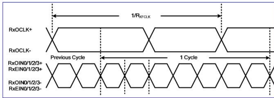
E. Fig. 7 Data skew margin Differential Input Data Format
