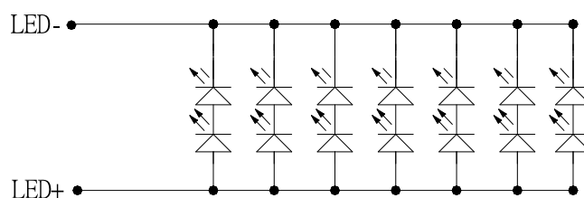
CIRCUIT DIAGRAM(2串7并)
