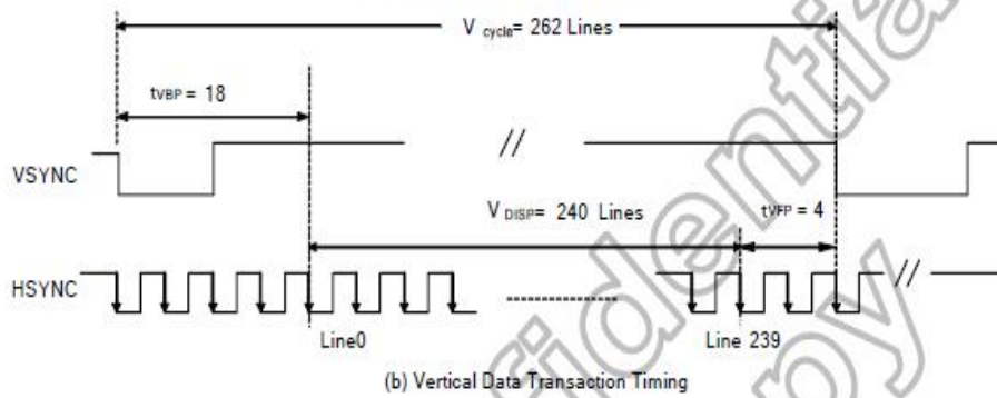
Figure 12. 2: Data transaction timing in parallel RGB (24-bit) interface (SYNC mode)
