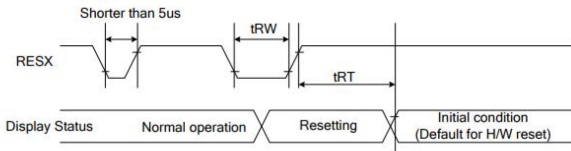
Figure 124: Reset Timing
