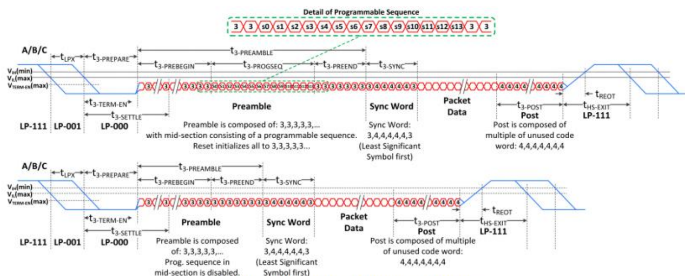
Figure: High Speed Data Transmission in Bursts
