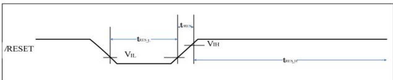
Reset timing
