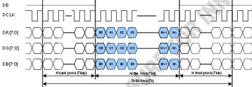
Parallel RGB input timing table
