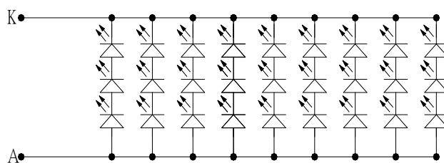
Backlight Circuit diagram
