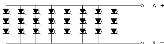
Figure: LED connection of backlight(Constant Current)
