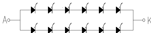
CIRCUIT DIAGRAM
