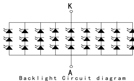
Figure: LED connection of backlight(Constant Current)
